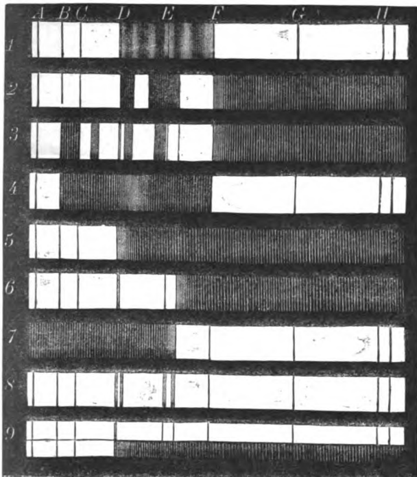
FIG. 5.—Absorption spectra.
